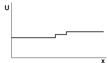
r / Making the step more gradual reduces the probability of reflection.
